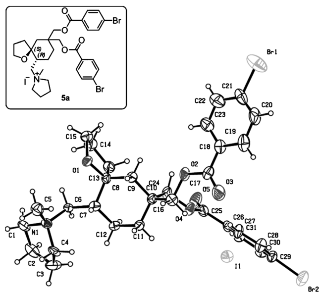
Figure 2. X-Ray crystallographic analysis of enantiopure 5a . Thermal ellipsoids are shown at 30% probability.
