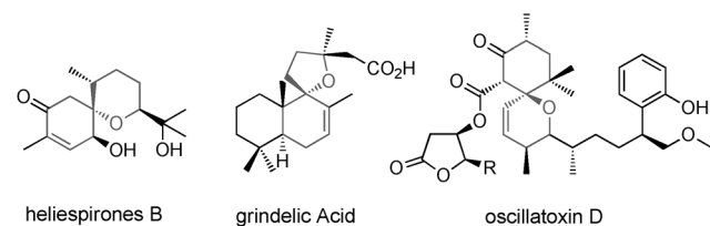
Figure 1. Natural products containing a spiroether moiety.
