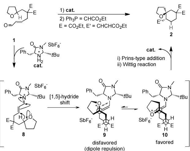
Scheme 3. Proposed mechanism of the redox reaction.
